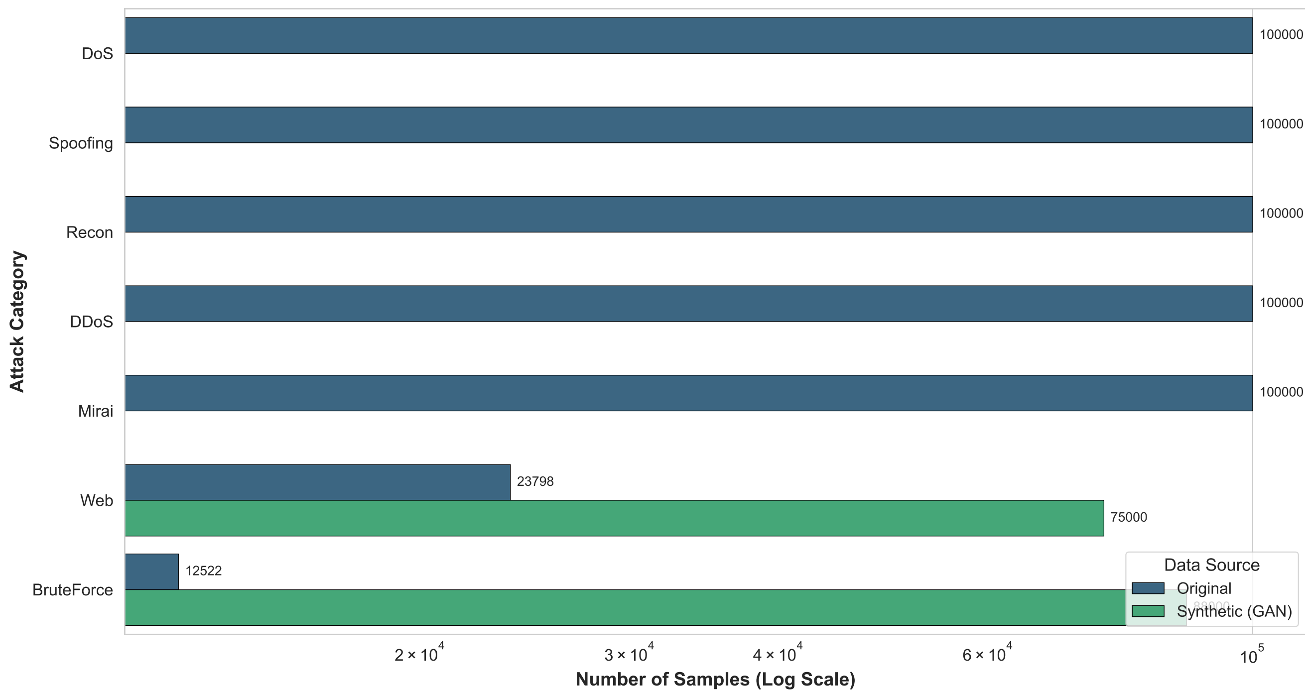
Distribution of Attack Classes: Original vs. Synthetic Data
