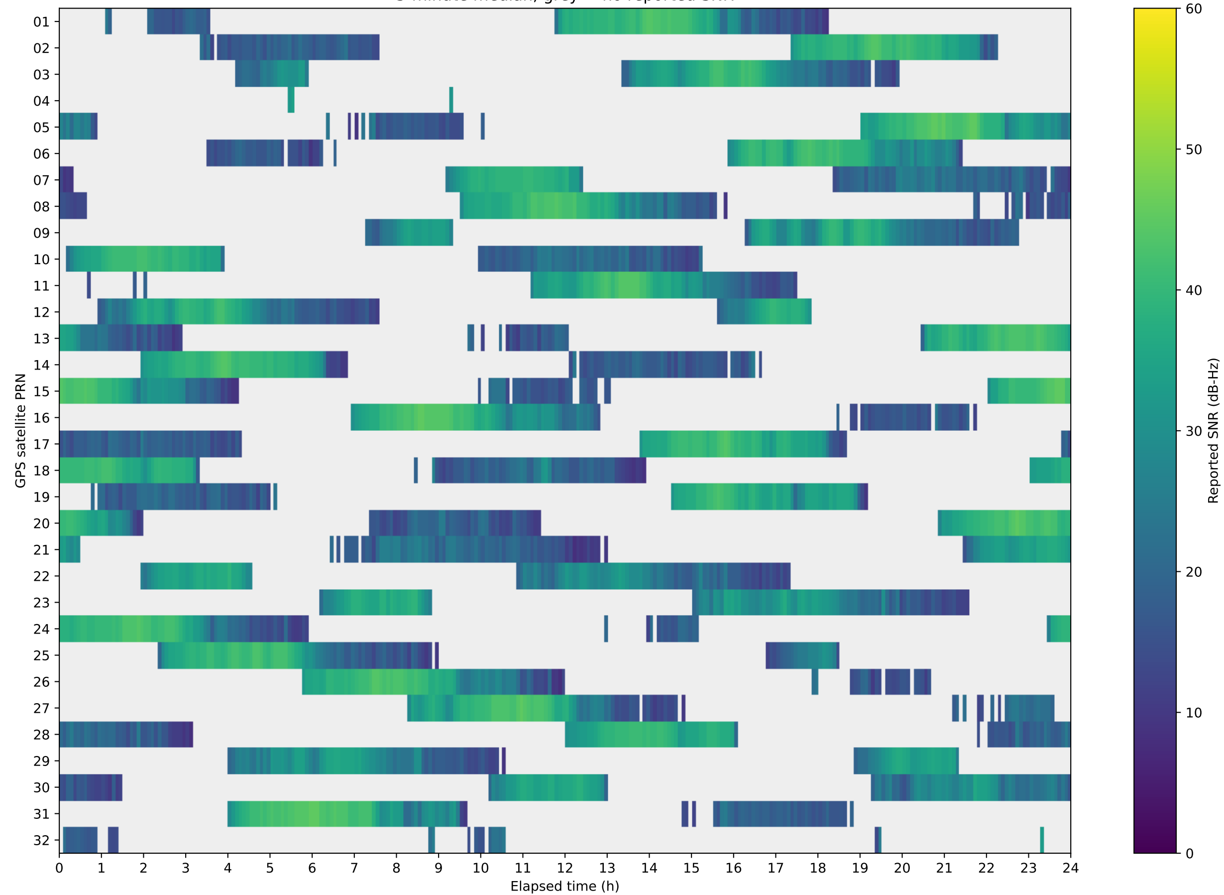
Satellite signal strength over 24 hours 5-minute median; grey = no reported SNR
