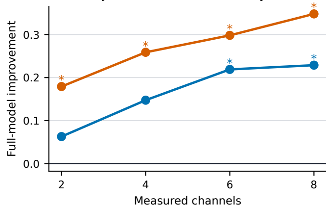
Uncertainty ablation: error-uncertainty association
