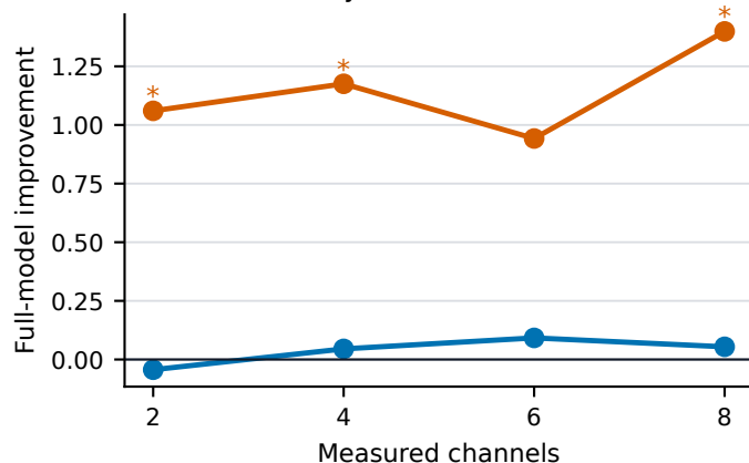
Uncertainty ablation: Gaussian NLL
