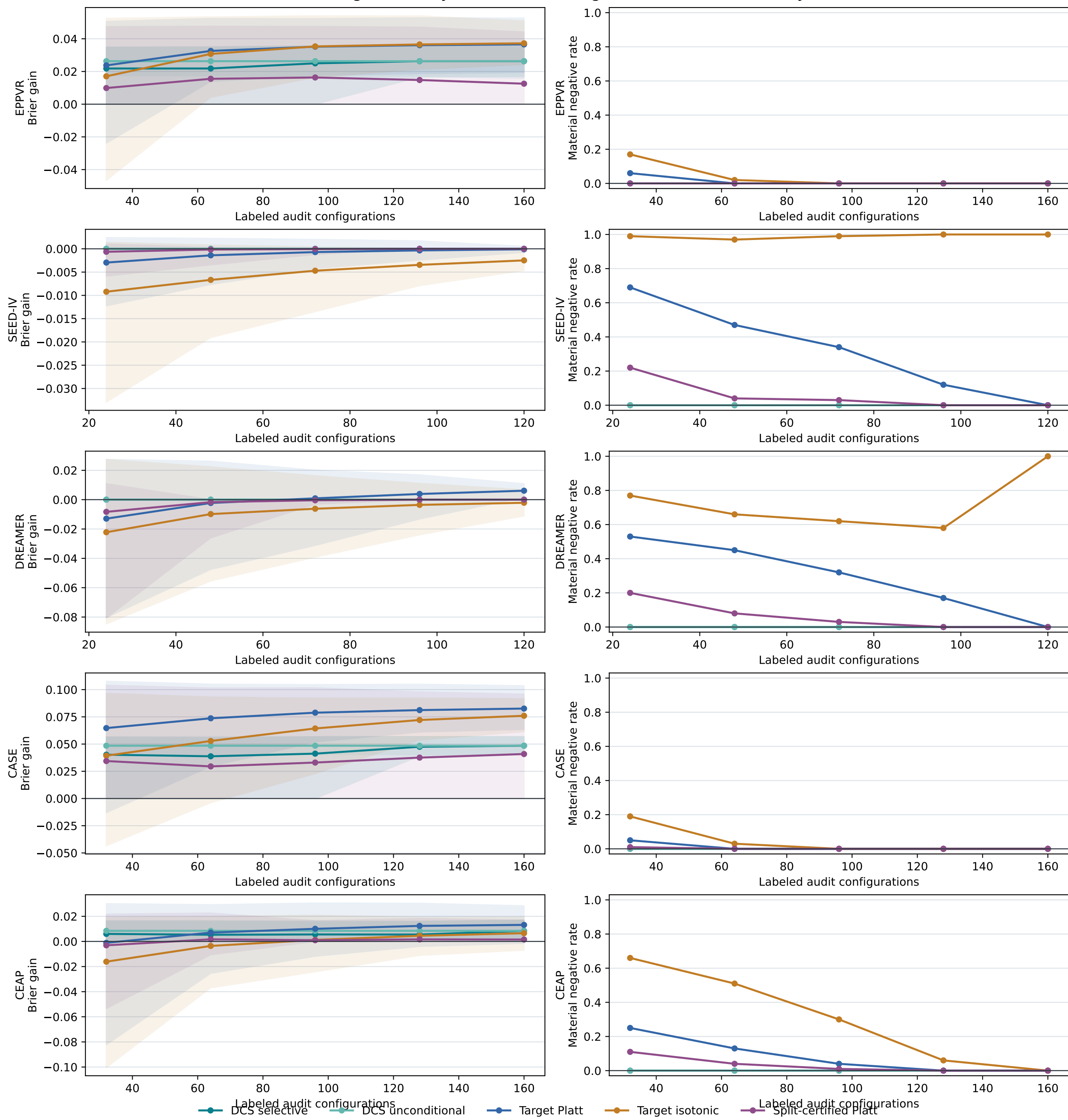
Audit-budget efficacy and material-negative-transfer sensitivity
