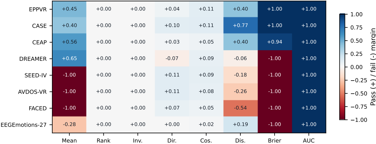
C Signed distance from each frozen gate (clipped normalized scale)
