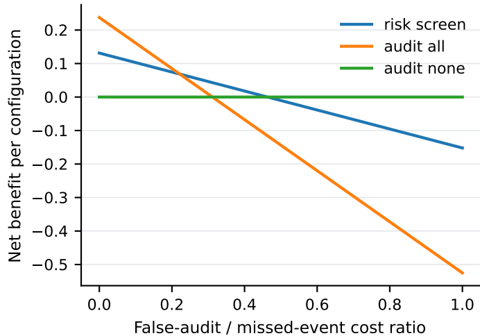
D Configuration-level decision curve at 0.02
