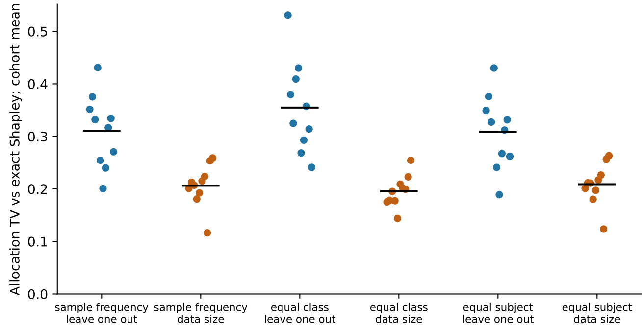
Exploratory scoring-reference comparison · points are seeds
