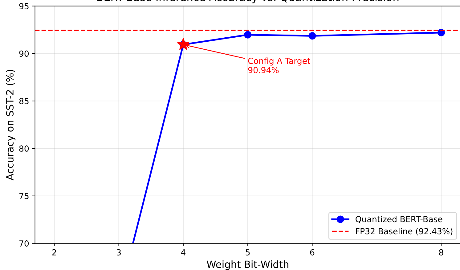
BERT-Base Inference Accuracy vs. Quantization Precision
