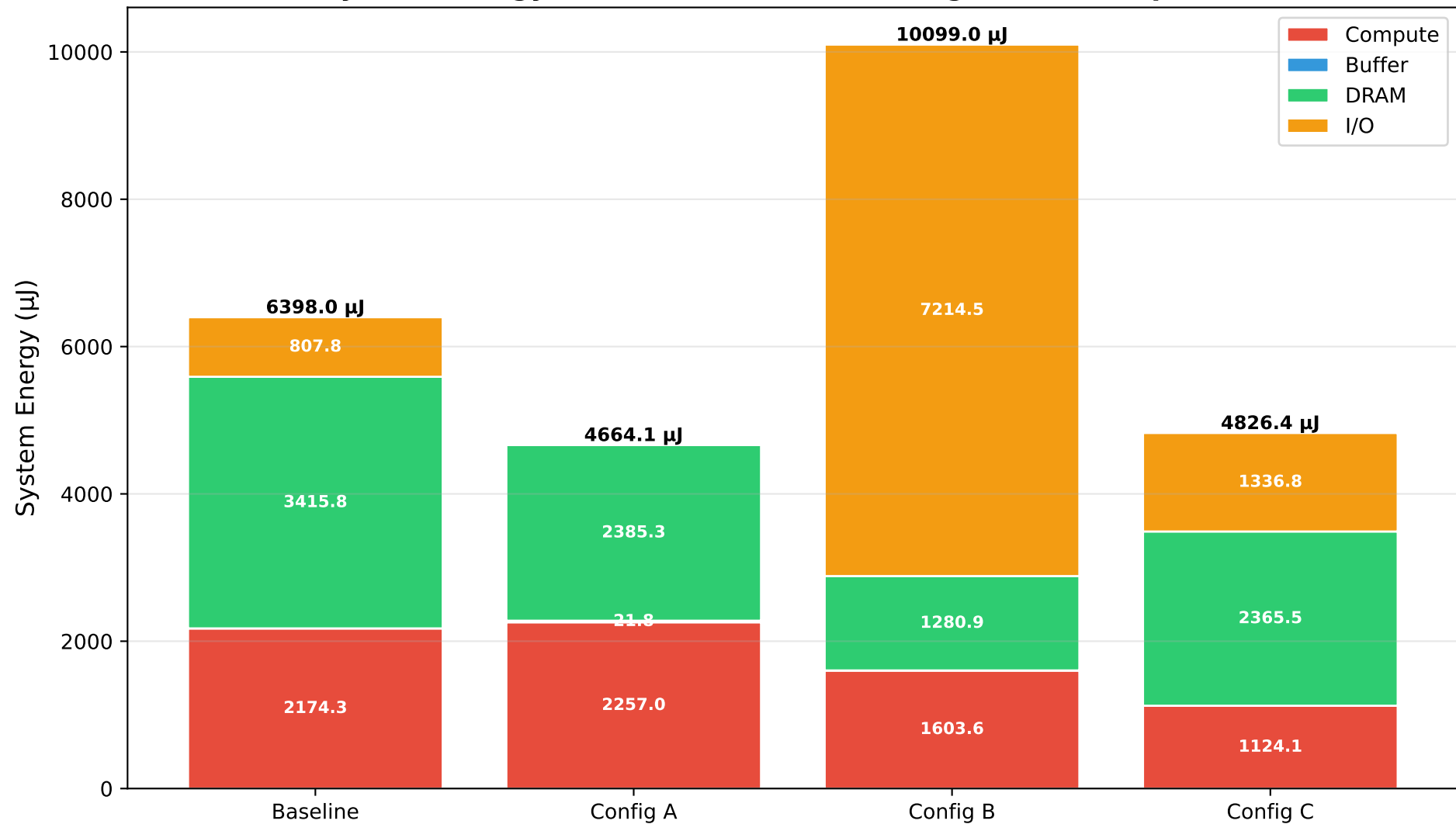
System Energy Breakdown — Cross-Configuration Comparison
