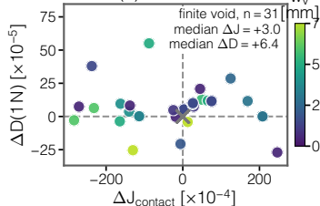
(c) Void Effect
