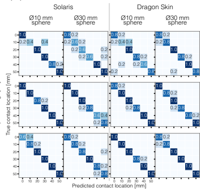
(c) Contact-location decoding
