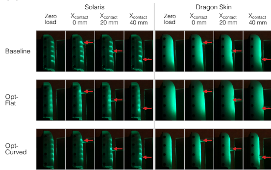
(a) Optical signatures across contact locations
