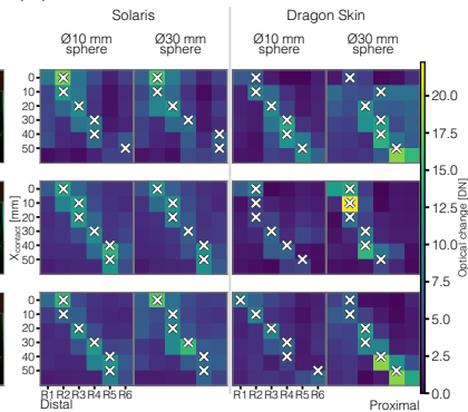
(b) Optical signal change, 2-15 N
