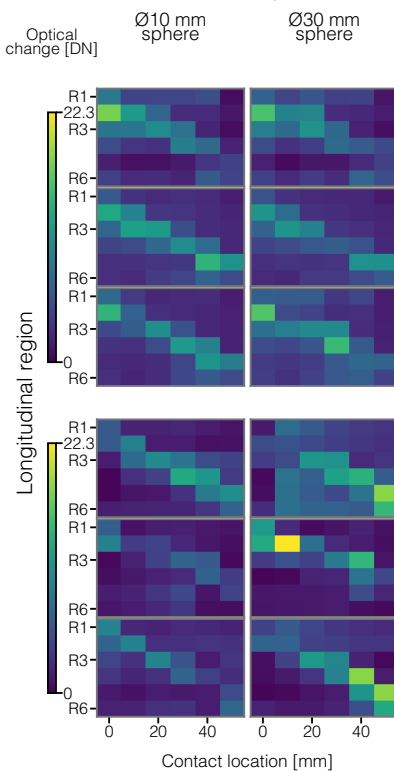
(b) Spatial optical response, 2–15 N Median of n = 5 re-contacts / location
