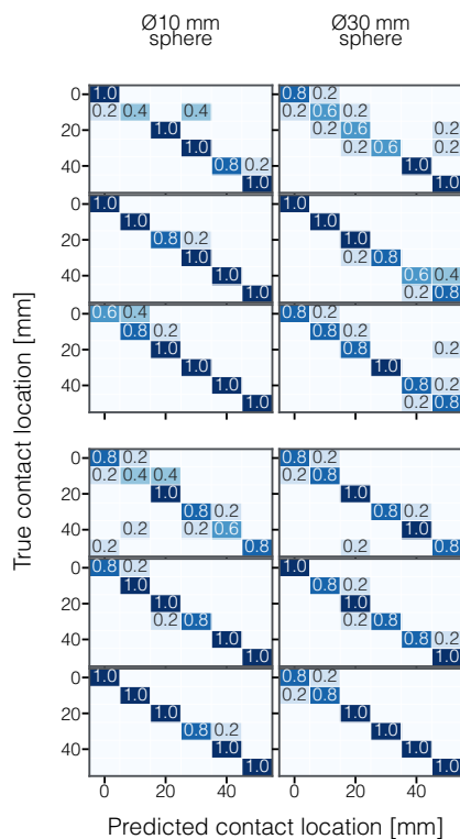
(c) Contact-location decoding n = 30 held-out predictions / matrix (5 / location)
