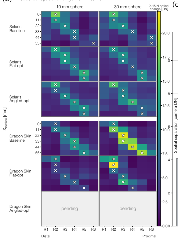
(b) Measured optical change from 2 to 15 N
