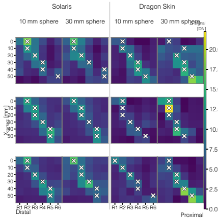
(b) Measured optical change from 2 to 15 N
