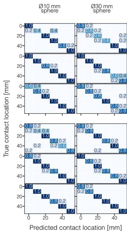
(c) Contact-location decoding
