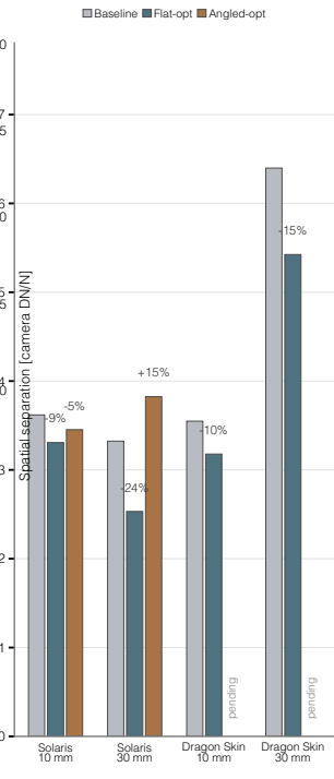
(c) Spatial separation across hardware conditions
