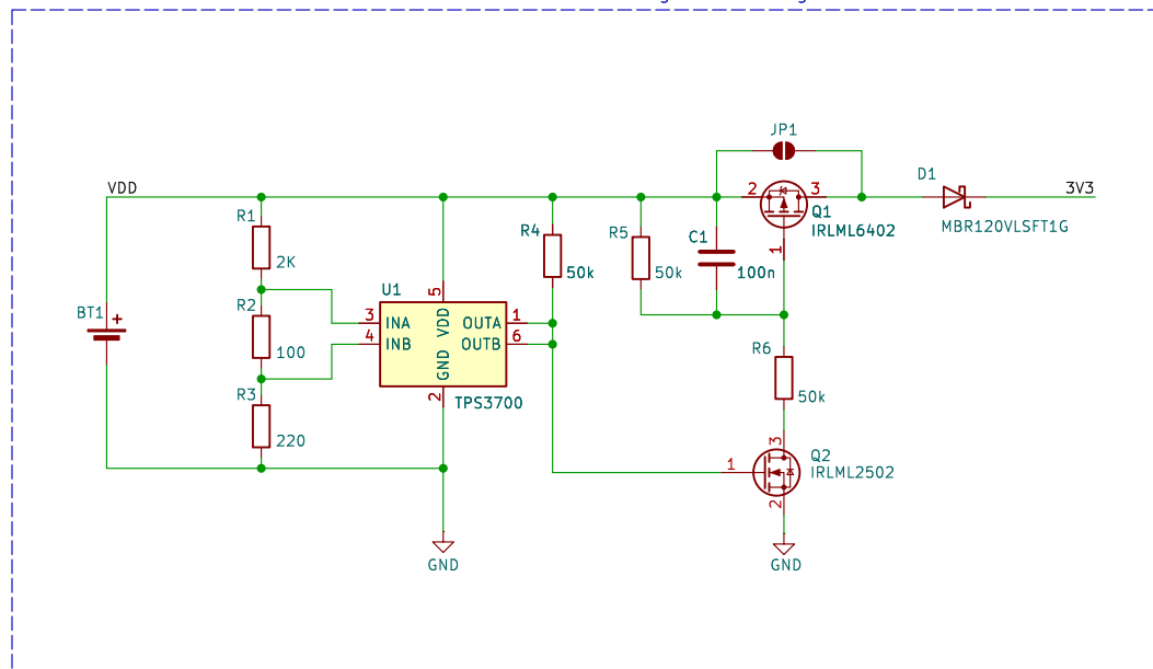
Over- and Undervoltage monitoring
