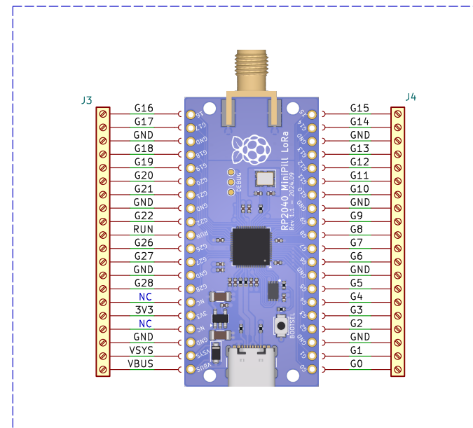
RP2040 MiniPill LoRa - Pinout
