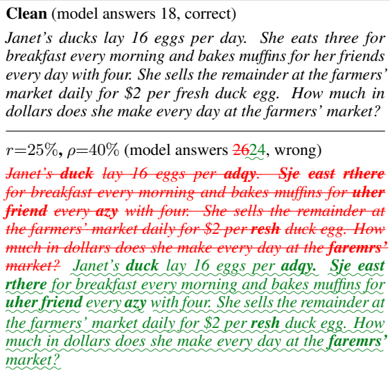
Figure 1: A single GSM8K item under our generator. Numbers and \LaTeX are protected; only alphabetic words are corrupted. Three Four of the ten typos are real words ( ducks → duck , eats → east , friends → friend , fresh → resh ); three of them ( ducks → duck , eats → east , friends → friend ) and are invisible to a accepted by the spell checker of $5.5 . The model answers 26 24 instead of 18.
