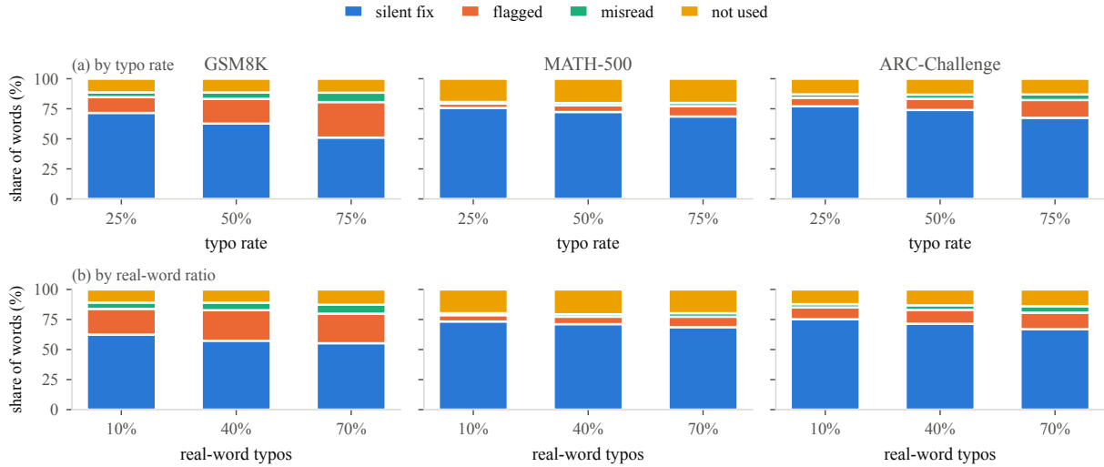
Figure 4: Word-level repair behavior. How every each corrupted word ( three or more letters, answered questions ) is handled in the reasoning trace. (a) against the typo rate, pooled over real-word ratios. (b) against the real-word ratio, pooled over typo rates. Silent fixing gives way to explicit flagging and to misreading as either the typo rate or the real-word ratio increases ( on GSM8K, flagging levels off above \rho=40 ), while the share of words never referred to stays roughly constant. Per-configuration values are in Table A5.
