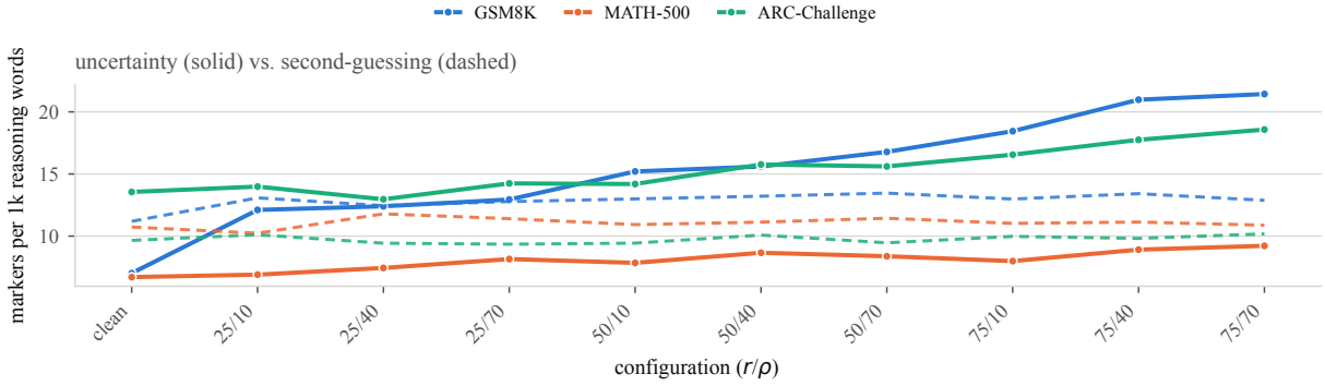
Figure 5: Self-doubt under typos. Marker density per 1,000 reasoning words across the grid. Uncertainty markers (solid) rise with corruption on all three datasets (on ARC only above r=25 ), most steeply on GSM8K, while second-guessing markers (dashed) stay roughly flat: typos make the model express much more doubt but verify only slightly more. The ratio of uncertainty density in wrong- to correct-answer traces is in Table A4.
