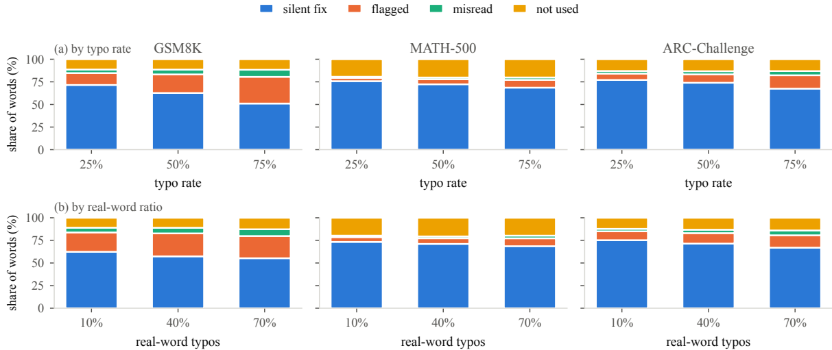
Figure 4: Word-level repair behavior. How each corrupted word (three or more letters, answered questions) is handled in the reasoning trace. (a) against the typo rate, pooled over real-word ratios. (b) against the real-word ratio, pooled over typo rates. Silent fixing gives way to explicit flagging and to misreading as either the typo rate or the real-word ratio increases (on GSM8K, flagging levels off above \rho=40 ), while the share of words never referred to stays roughly constant. Per-configuration values are in Table A5.
