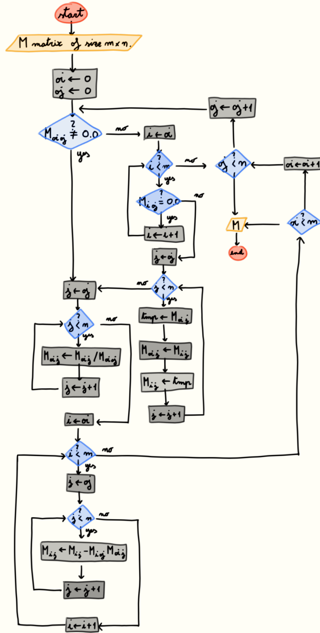
Figure 10: Formalized diagram of the previous row reduction algorithm implementation.
