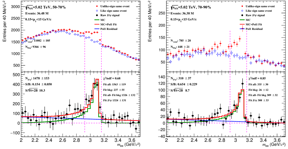
Figure 15: The p_T integrated J/\psi signal extraction performance with the standard cuts, the background shape from the same event like-sign, different panel for different centralities.
