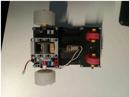
Final robot, bottom
