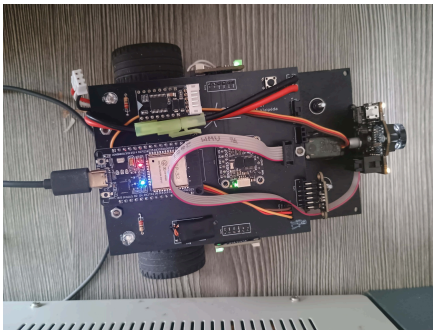
Installed sensor positions. Left and right VL53L1X modules sit at the PCB side edges; the front VL53L1X is beside Pixy2.
