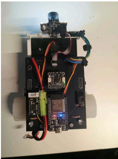
Final robot, top
