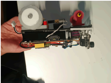
Final robot, right side
