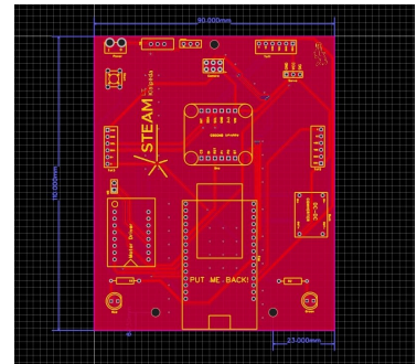
PCB footprint. The drawing marks the board as 90 × 100 mm.
