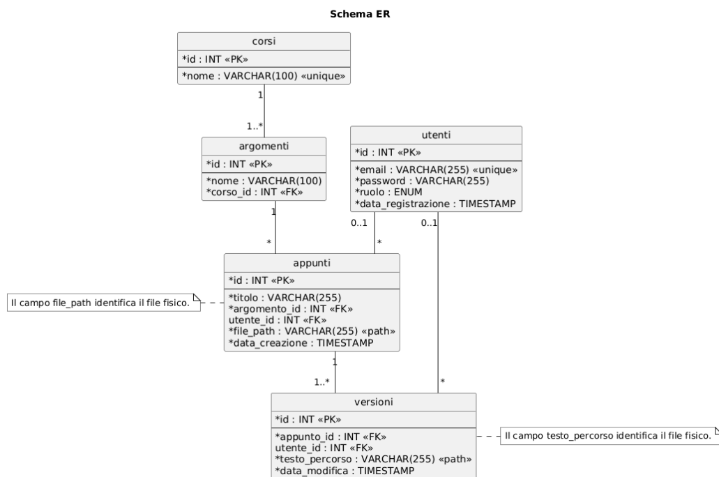
Figura 5.8: Schema Entity-Relationship
