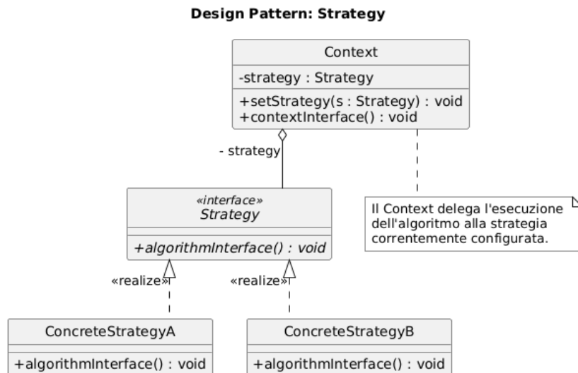
Figura 6.3: Strategy
