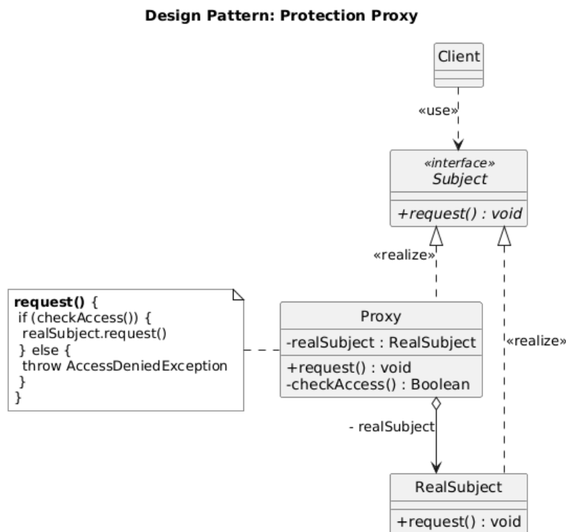
Figura 6.5: Protection Proxy
