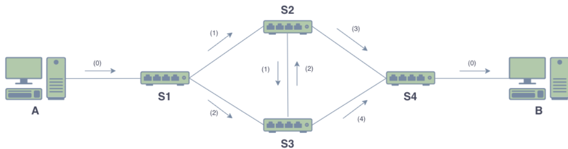
Figura 1.5: Flusso da host A ad host B mediante switch S1-S4
