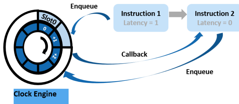
Figure 3.2: GVSoC Event Engine
