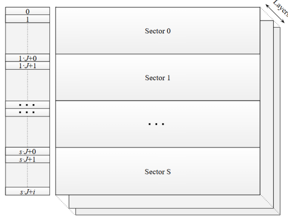
Figure 3.3: PCM matrix data-structure after cache-friendliness optimisation.
