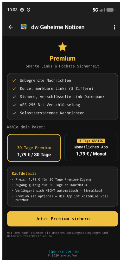
Der Premium-Upgrade-Bildschirm
