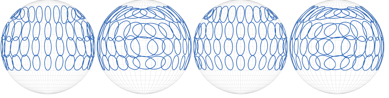
Fig. 1. Local auditory discrimination ellipses derived from the Cramér-Rao bound. Ellipses show the 95% contour of a bivariate Gaussian with covariance equal to the CRB, scaled by \sqrt{\chi^2_{2,0.95}} . Views correspond to azimuths of 0^\circ , 90^\circ , 180^\circ , and 270^\circ . Results are based on the median Fisher tensor of the 41-subject SONICOM evaluation cohort.
