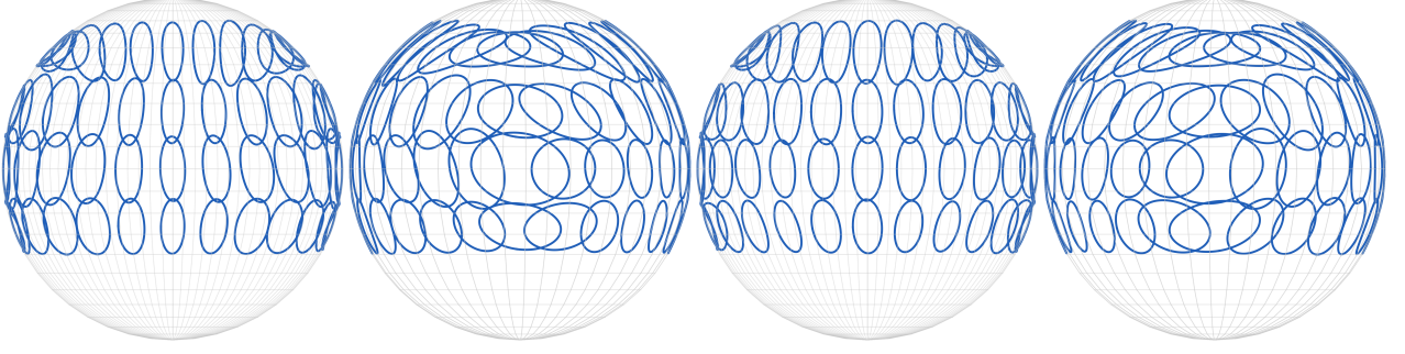
Fig. 2. Local auditory discrimination ellipses derived from the Cramér-Rao bound. Ellipses show the 95% contour of a bivariate Gaussian with covariance equal to the CRB, scaled by \sqrt{\chi^2_{2,0.95}} . Views correspond to azimuths of 0^\circ , 90^\circ , 180^\circ , and 270^\circ . Results are based on the median Fisher tensor of the 41-subject SONICOM evaluation cohort.
