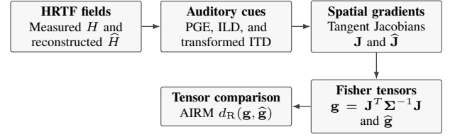
Fig. 1. Evaluation pipeline for comparing measured and reconstructed HRTF fields through their local auditory-cue sensitivity.
