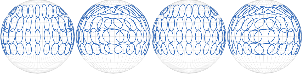
Fig. 2. Local auditory discrimination ellipses derived from the Cramér-Rao bound. Ellipses show the 95% contour of a bivariate Gaussian with covariance equal to the CRB, scaled by \sqrt{\chi^2_{2,0.95}} . Views correspond to azimuths of 0^\circ , 90^\circ , 180^\circ , and 270^\circ . Results are based on the median Fisher tensor of the 41-subject SONICOM evaluation cohort.
