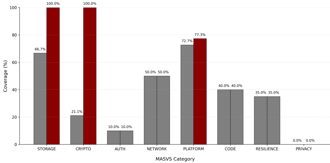
Figure 6.2.: Contribution of our apps to the relative coverage of MASWE vulnerabilities
