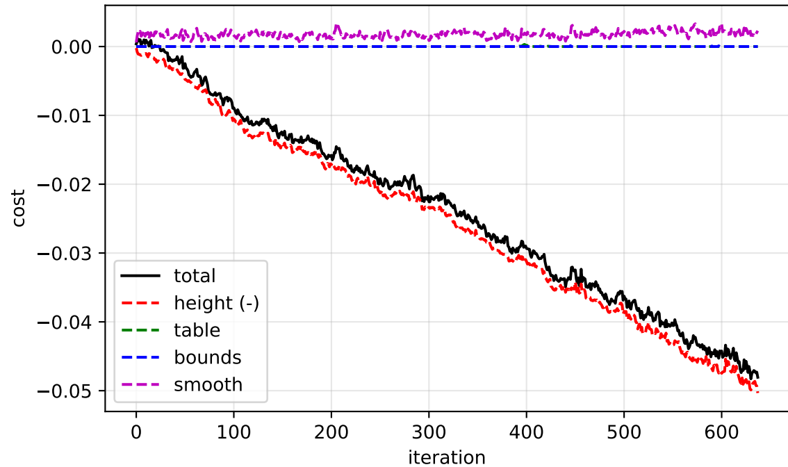
Cost trace
