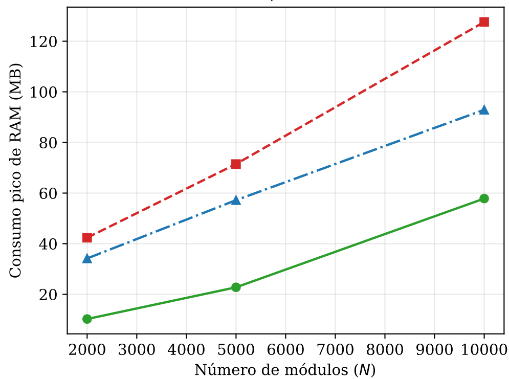
2048 bits, WEAK=100
