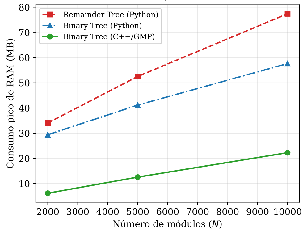
2048 bits, WEAK=2
