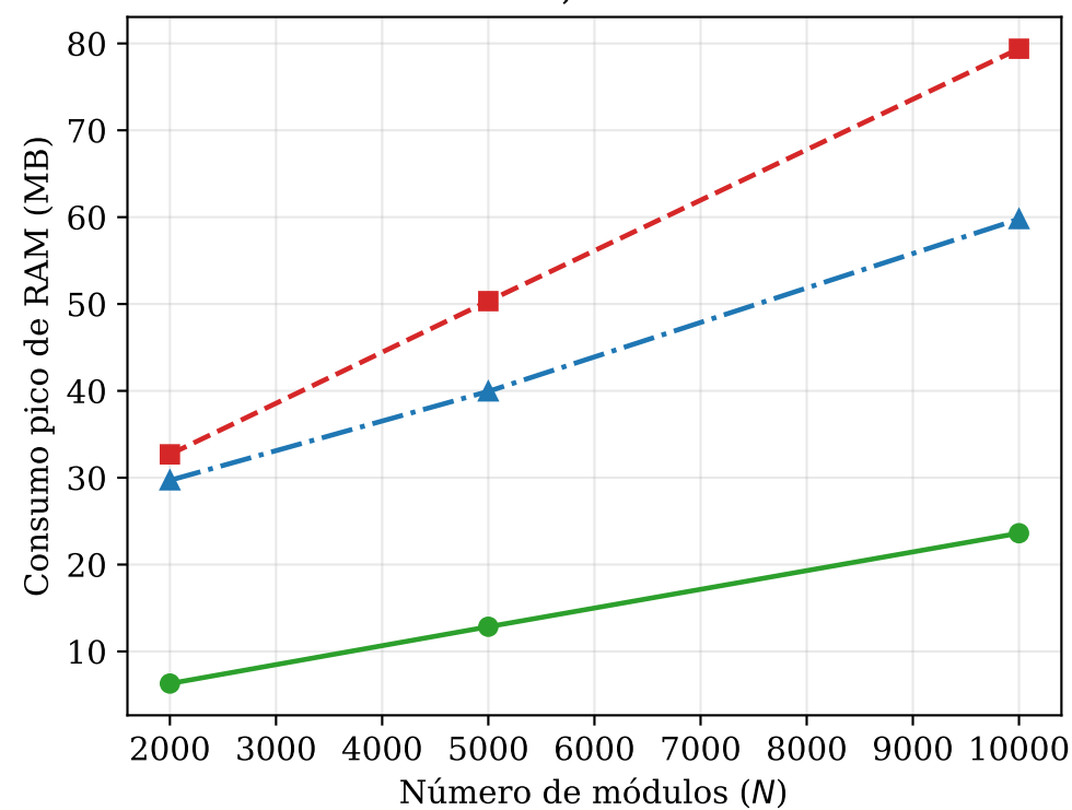
2048 bits, WEAK=100
