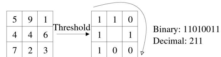
Fig. 1. The basic LBP operator.
