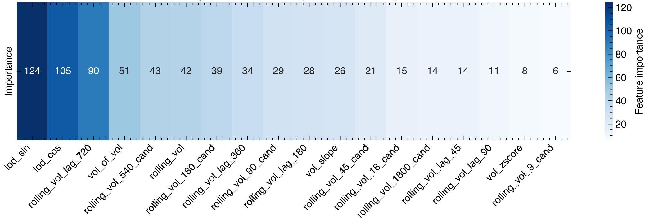
LightGBM Feature Importance Heatmap
