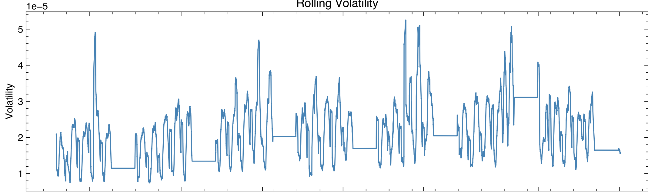
Future Rolling Volatility
