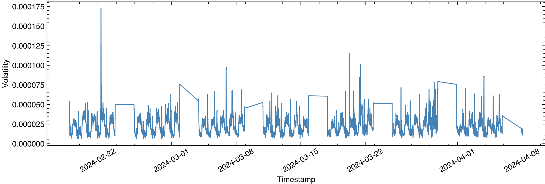
Future Rolling Volatility
