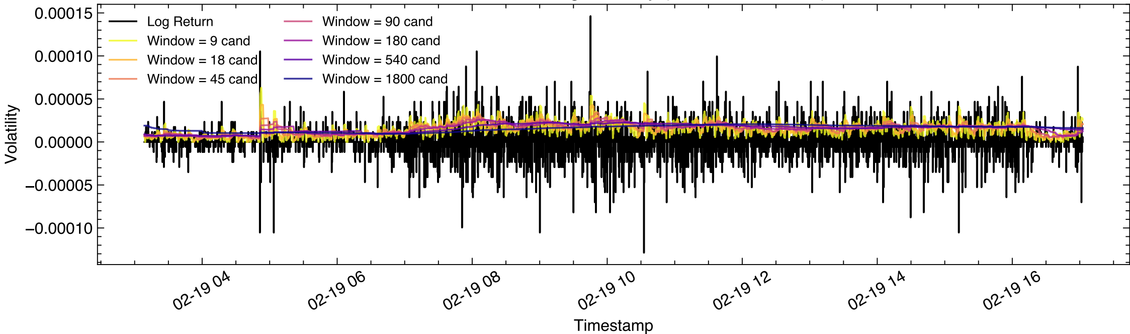
Multi-Window Rolling Volatility (first 5000 candles)
