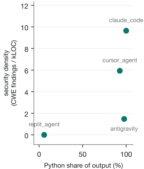
Why Replit scores 0.00
