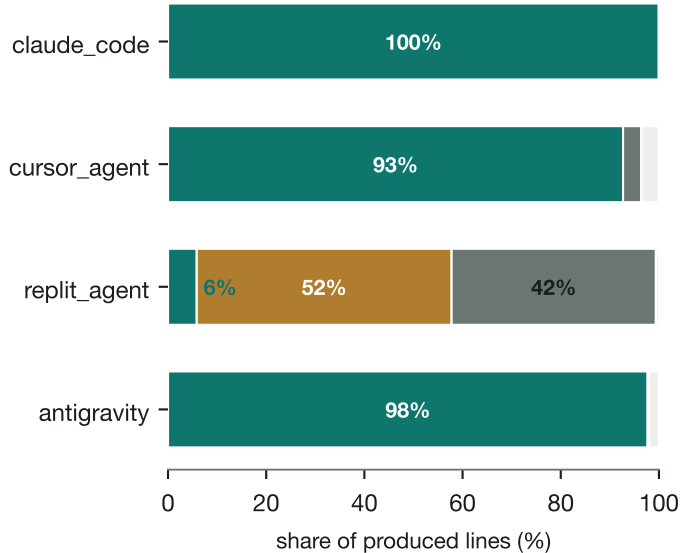
What each tool actually wrote
