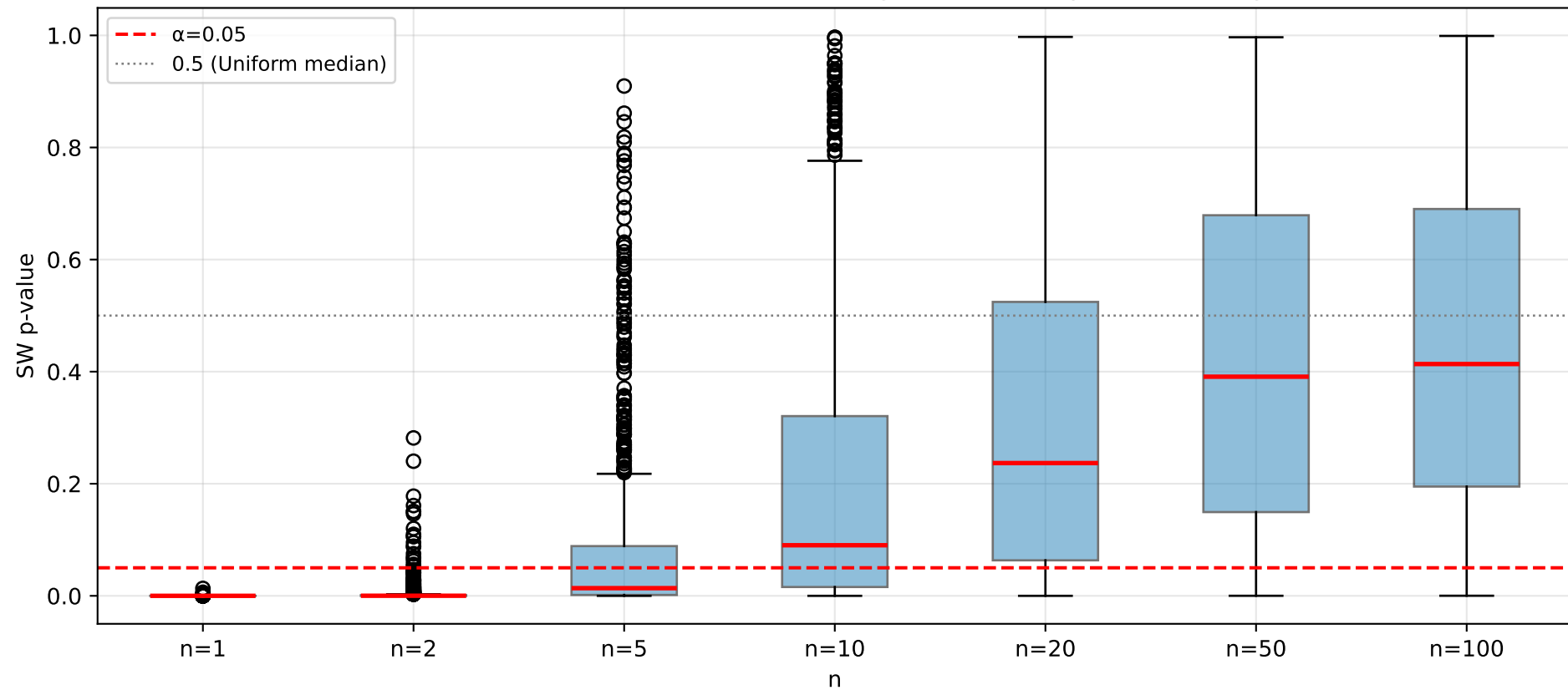
F3 - SW p-value distribution (1000 MC reps) Concentrated near 0 for small n (strong detection); spreads for large n
