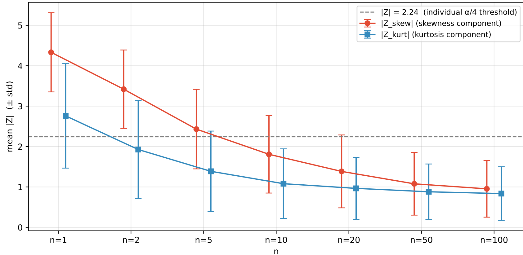
G3 - D'Agostino sub-statistics: skewness vs kurtosis component Both decay toward 0; skewness dominates at moderate n
