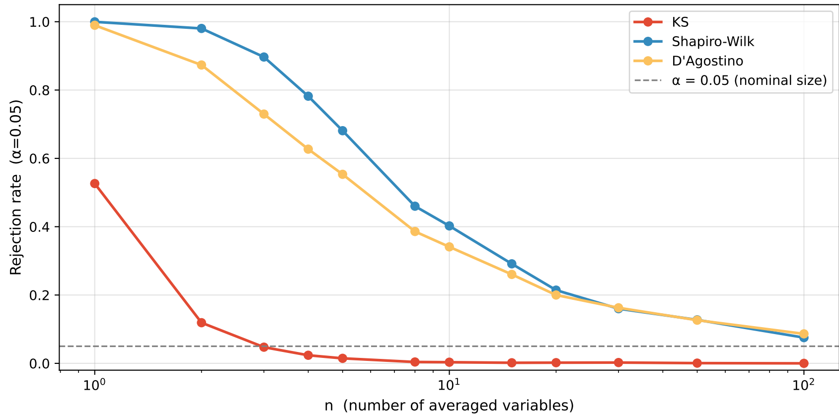
Power / empirical rejection rate Exponential( \lambda=1 ), K=60 means, 3000 MC reps
