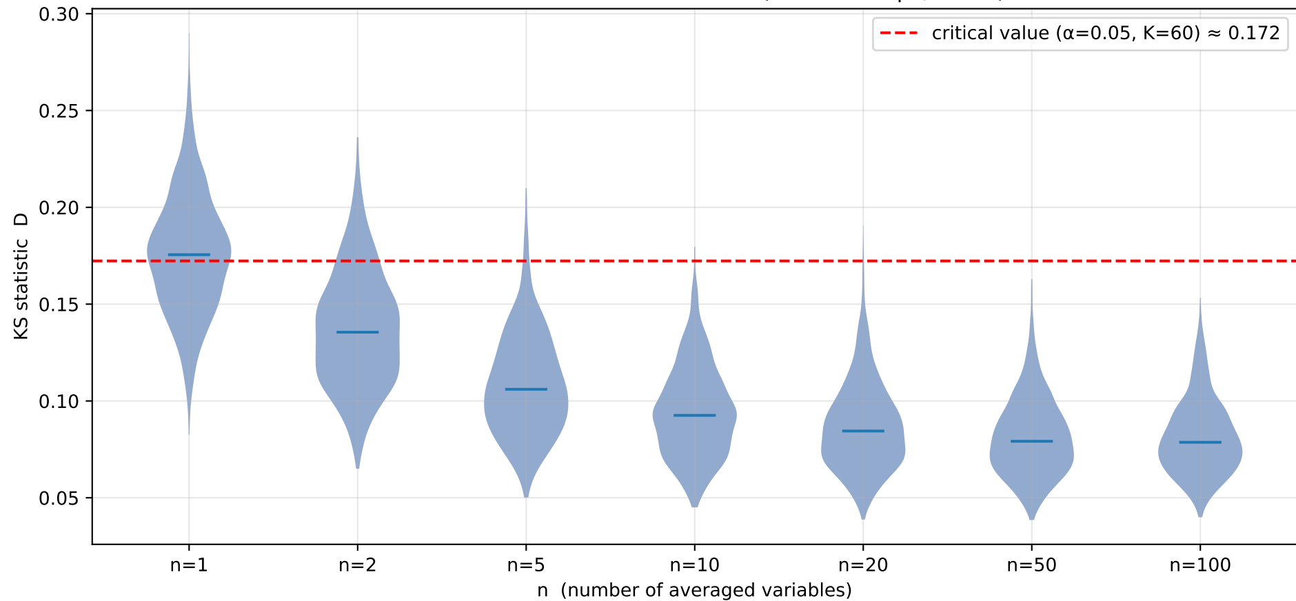
E2 - Distribution of KS statistic D (1000 MC reps, K=60)
