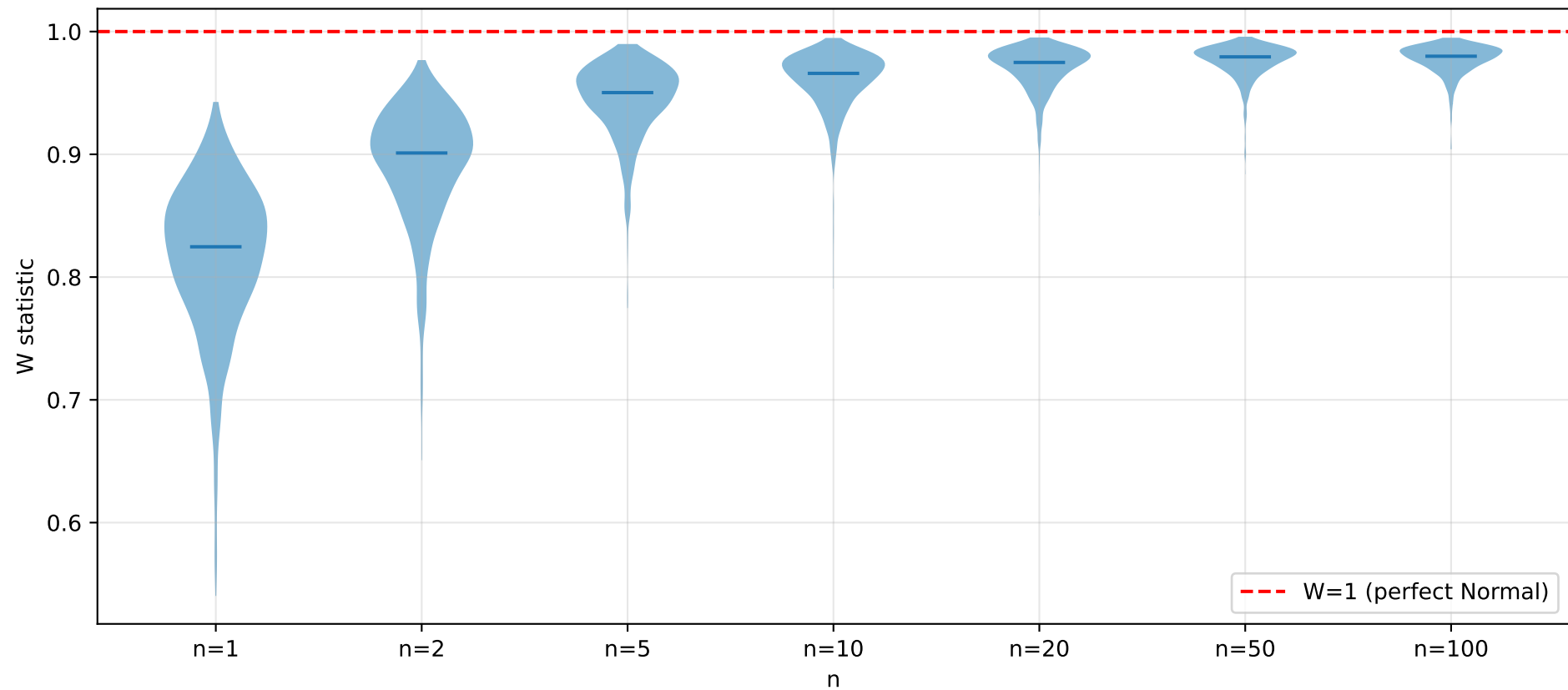
F2 - Distribution of SW W statistic (1000 MC reps, K=60) Median W \rightarrow 1 and variance shrinks as distribution becomes Normal
