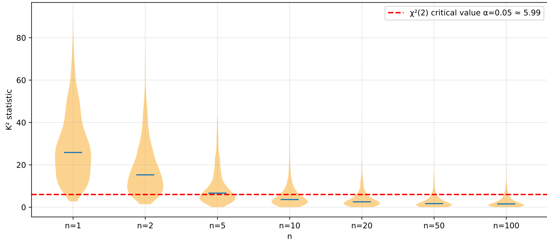
G2 - D'Agostino K^2 statistic distribution (1000 MC reps) Bulk shifts below critical value as distribution becomes Normal
