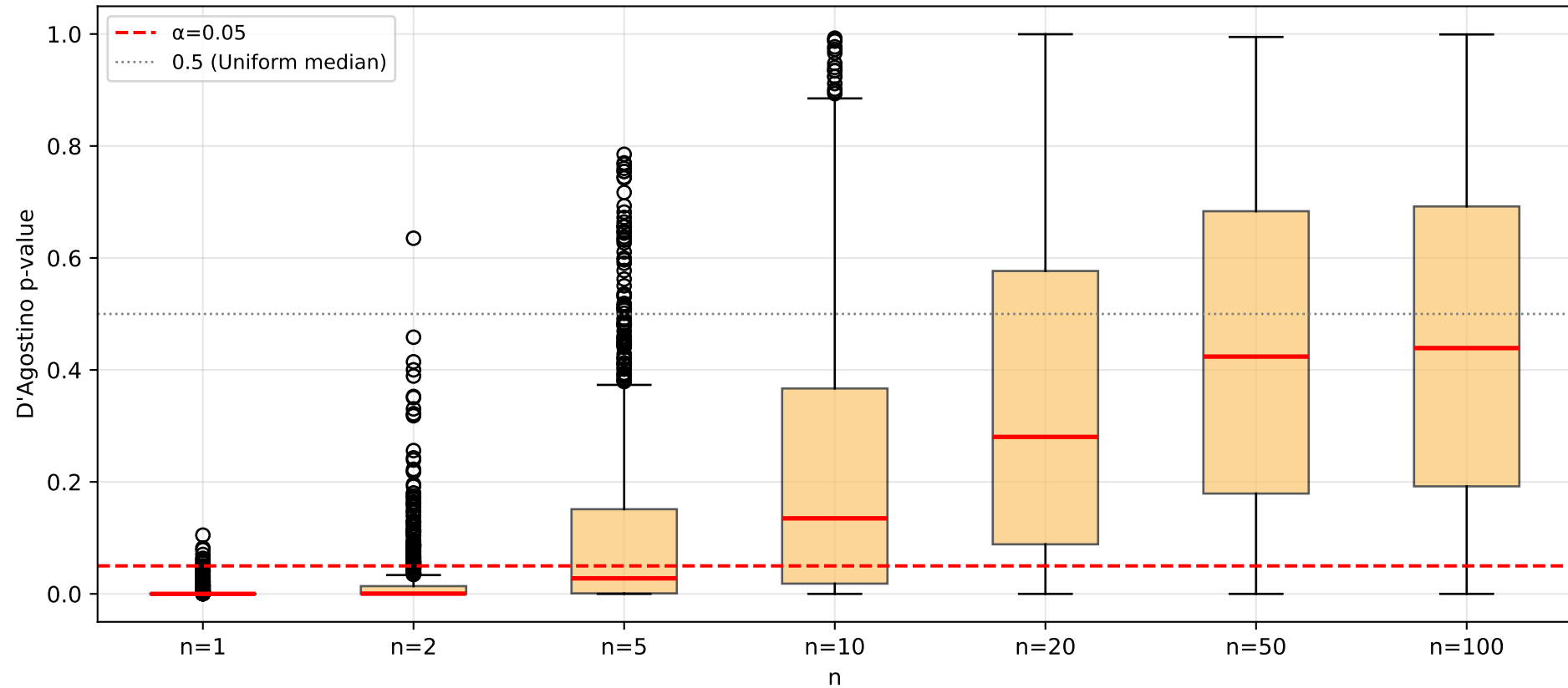
G4 - D'Agostino p-value distribution (1000 MC reps) Piles up near 0 for non-Normal data; spreads uniformly once Normal
