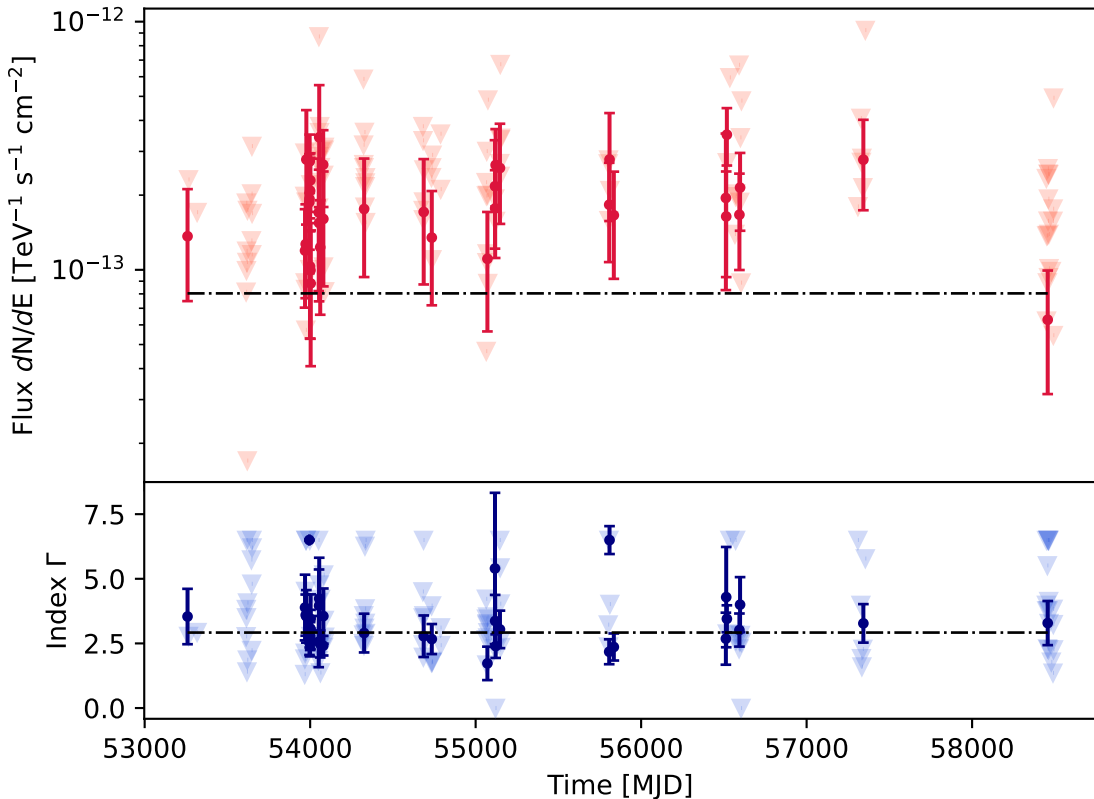
1ES0229+200 Light Curve
