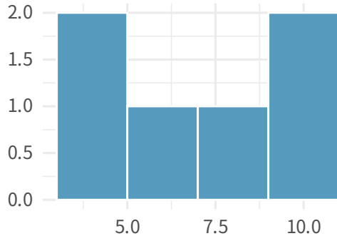
sixth
