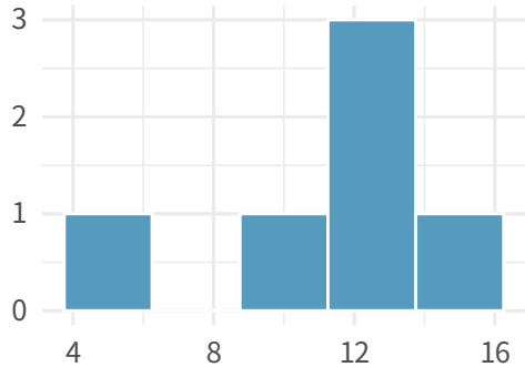
thirteenth
