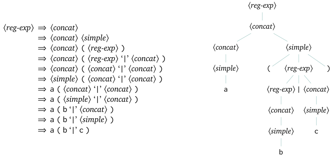
FIGURE 94, FOR QUESTION IV.3.35: Derivation and parse tree for a(b|c) .
