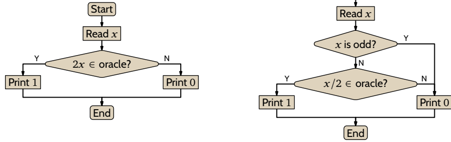
FIGURE 42, FOR QUESTION II.8.26: Showing that B \leq_T 2B and 2B \leq_T B .
