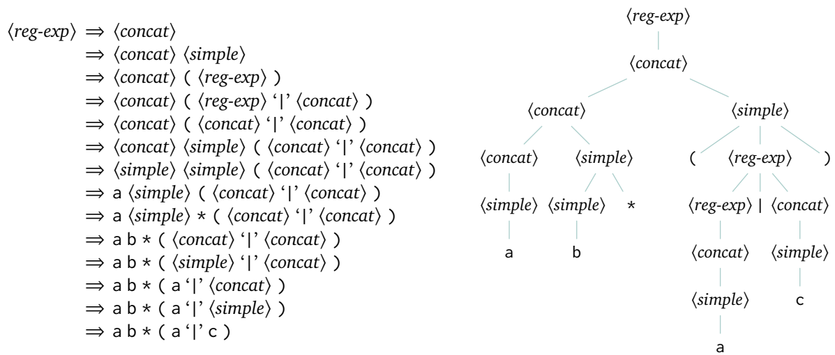
FIGURE 95, FOR QUESTION IV.3.35: Derivation and parse tree for ab^*(a|c) .
