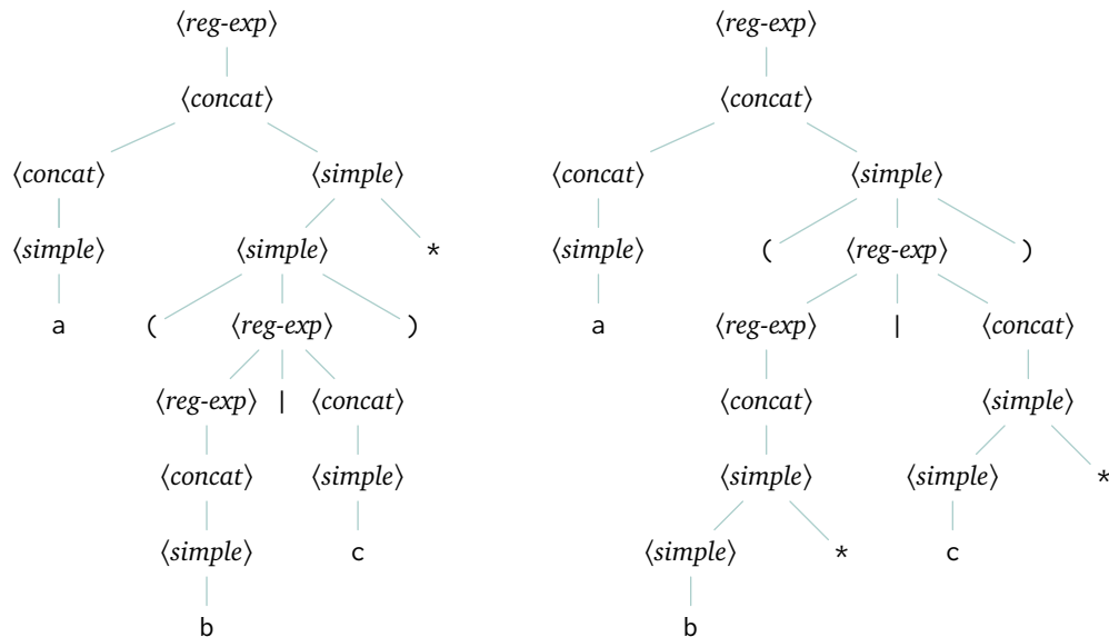
FIGURE 96, FOR QUESTION IV.3.36: Parse trees for a(b|c)^* and a(b^*|c^*) .
